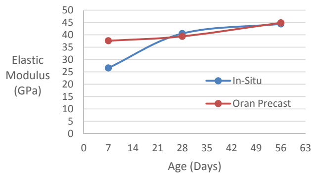
Figure 7. Development of elastic modulus with age for concrete mixes
