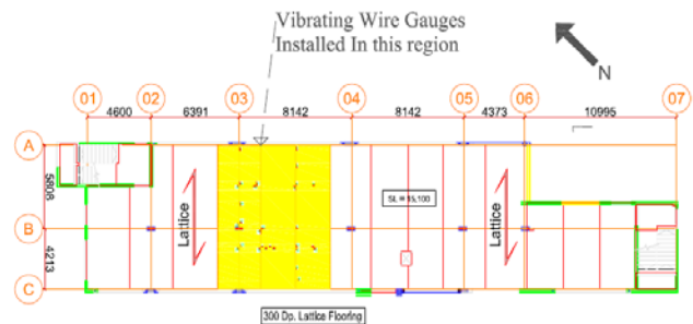
Figure 3. Plan of first floor of the East block of LCSi with instrumented area highlighted (dimensions in mm).
