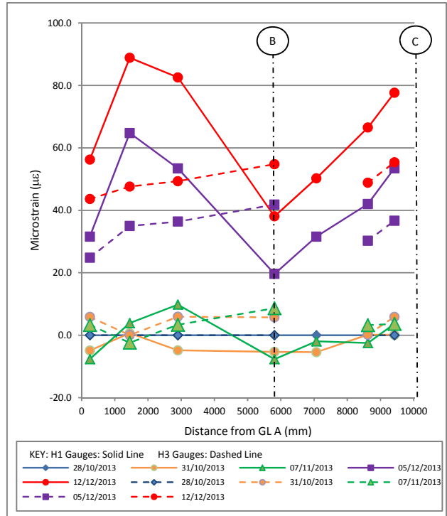
Figure 9. Changes in measured strain along GL 3.5
