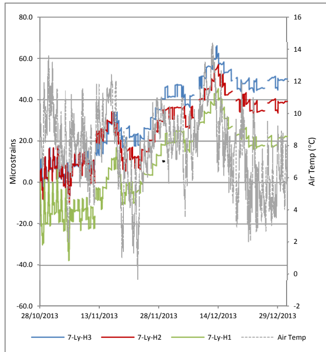
Figure 10. Measured strain (7-Ly) and air temperature
