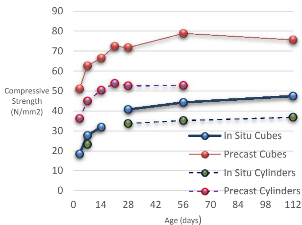
Figure 6. Development of average compressive strength with age
