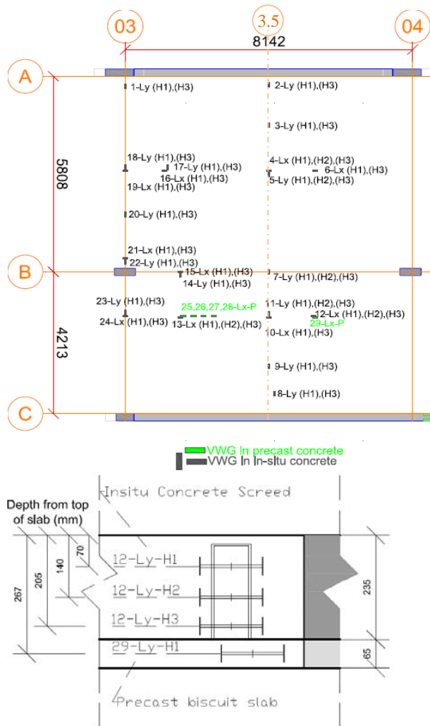
Figure 4. (a) Plan view and (b) typical section showing locations of vibrating wire gauge installed in the flat slab system (dimensions in mm).
